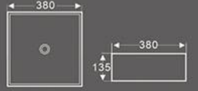
BA-185 Art Basin Size: 380x380x135 mm Vitreous china Above counter mounting
