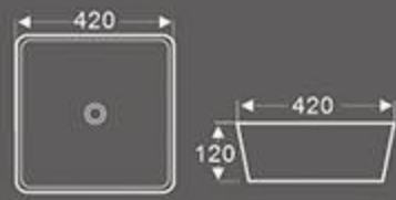
BA-057 Art Basin Size: 420x420x120 mm Vitreous china Above counter mounting
