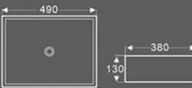
BA-069 Art Basin Size: 490x380x130 mm Vitreous china Above counter mounting
