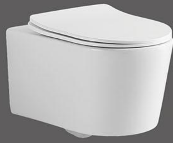
TW-020 Wall-hung Toilet Rimless washdown flushing Size: 530x360x390mm P trap: 180mm
