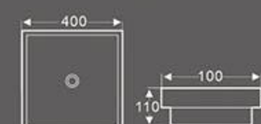
BA-131A Art Basin Size: 400x400x110 mm Vitreous china Above counter mounting
